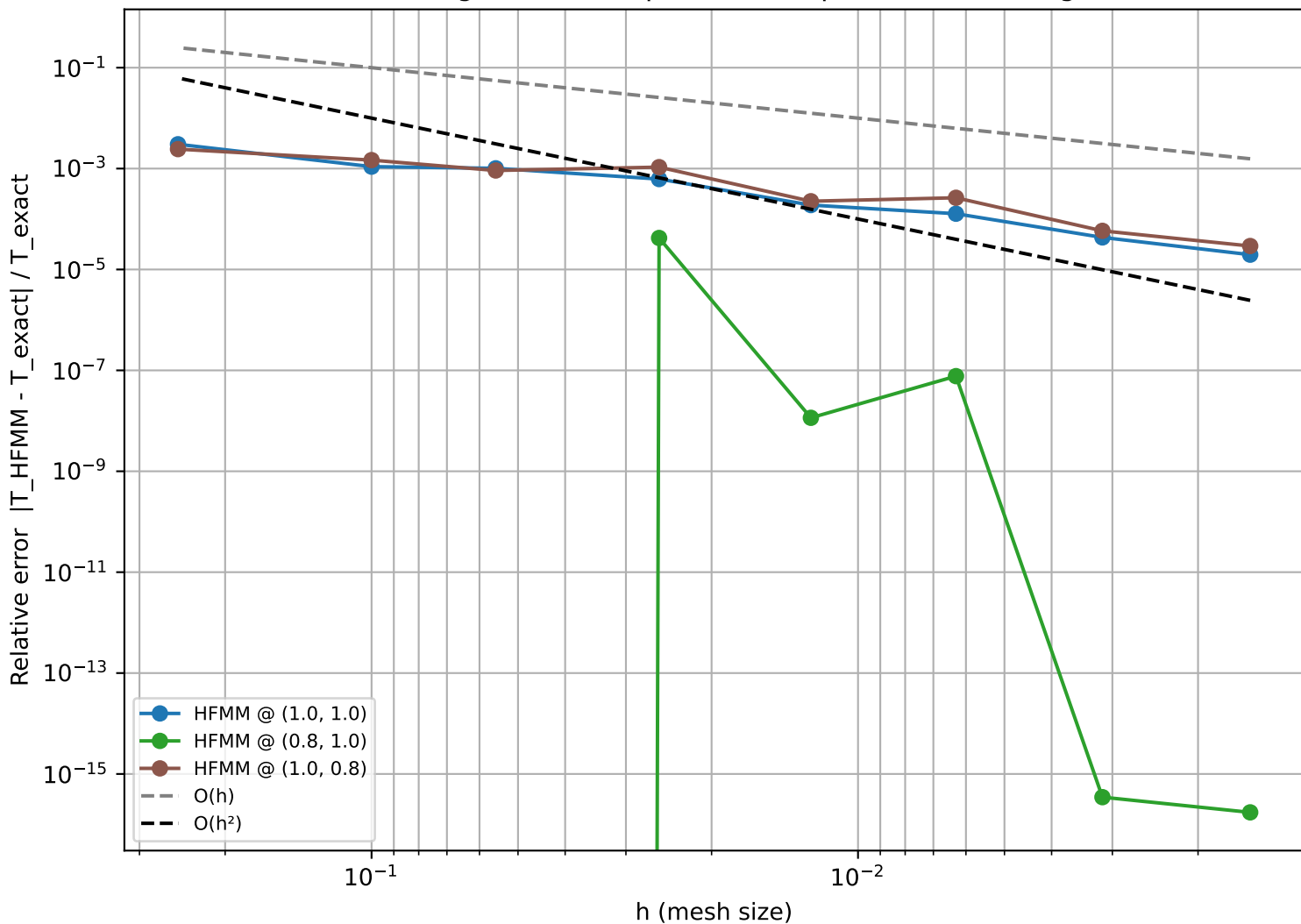
FMM Convergence - L-shape — HFMM pointwise convergence
